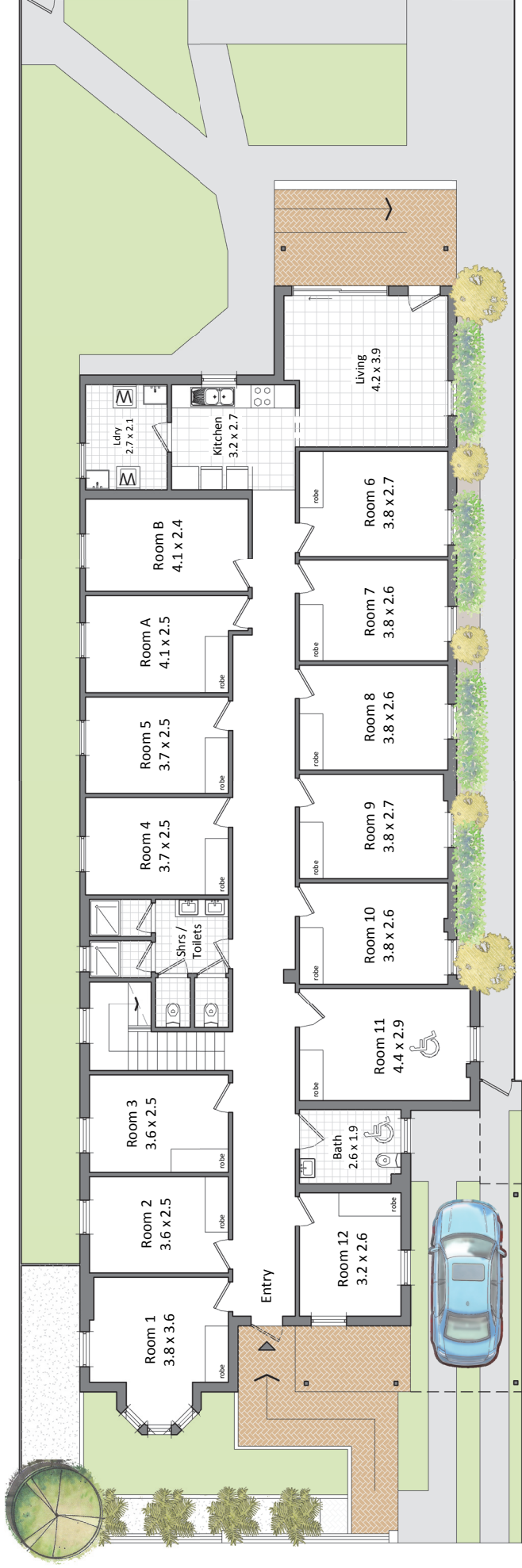
Ground level floor plan
